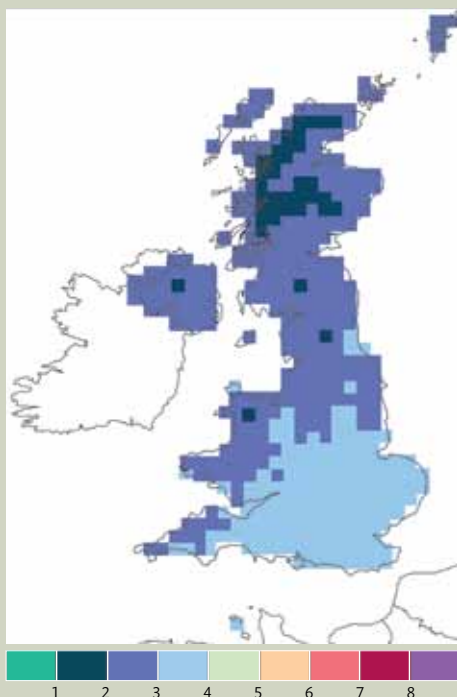
Forest fire danger index 1970–2000
