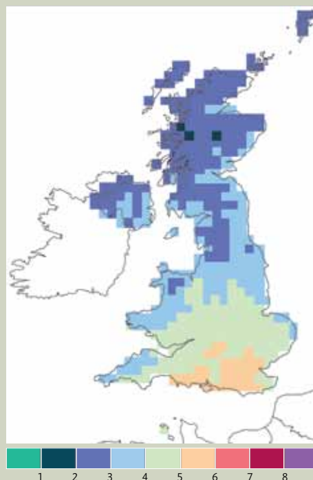
Forest fire danger index 2070–2100
