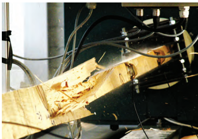
Figure 26 A softwood batten breaking during a laboratory torsion test.
