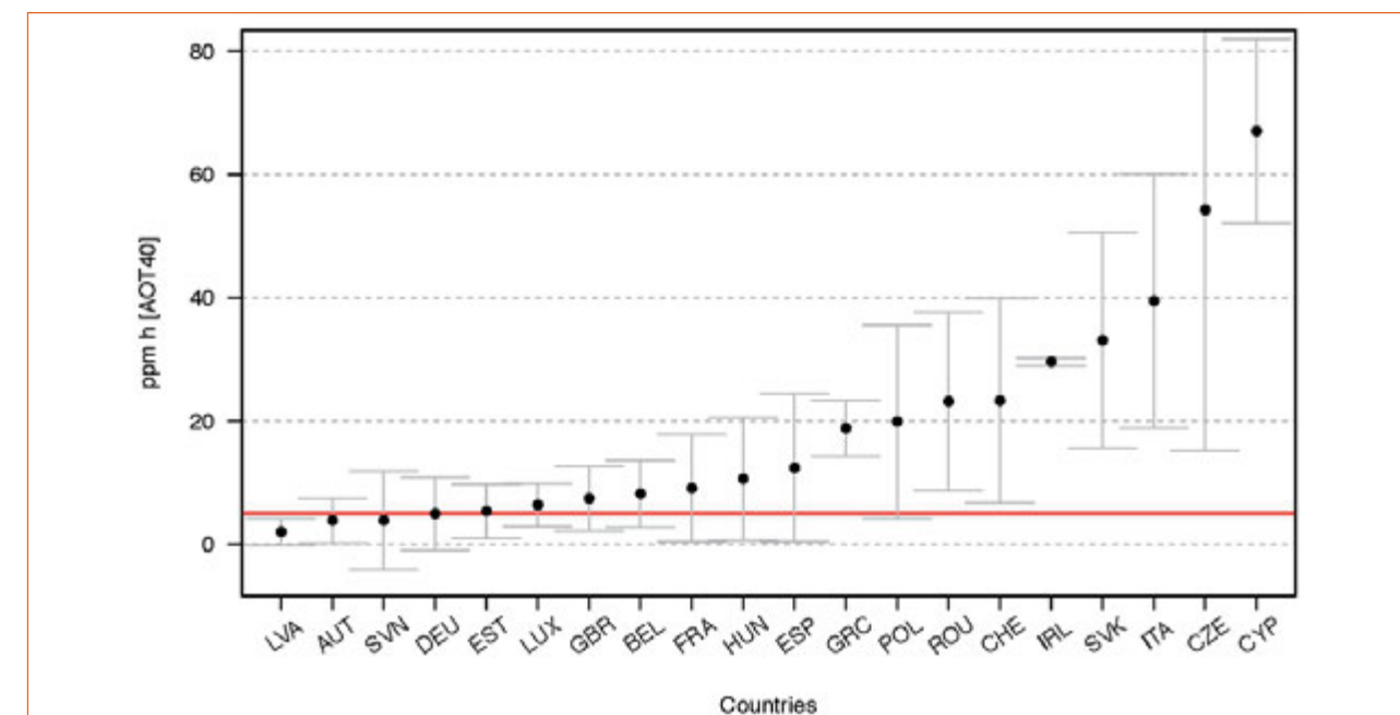
Figure 4.2. Mean AOT40 (ppm h) for 20 countries based on April - September passive ozone concentration values from 2000 to 2013. The red line identifies the Critical Level of 5 ppm h set to protect forest trees.
