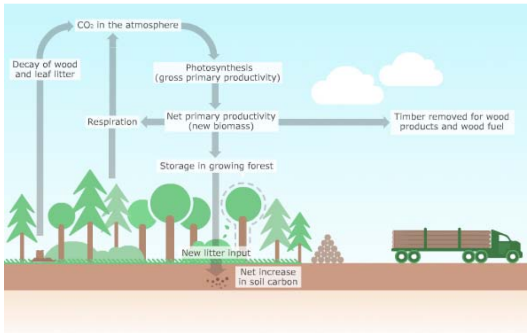
Figure 4.1 Carbon Cycle
