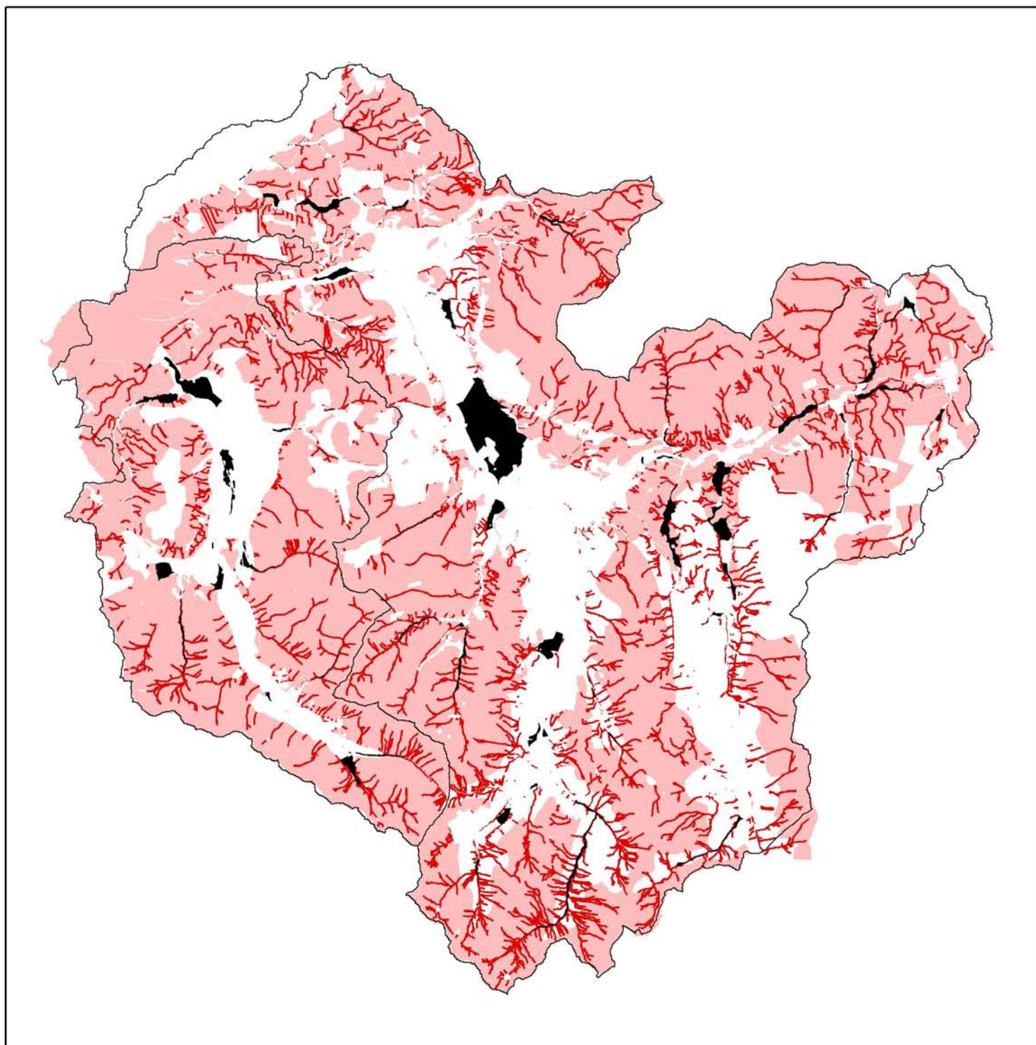
Map 20 Combined map showing high priority areas for floodplain, riparian and wider woodland creation to reduce downstream flooding
