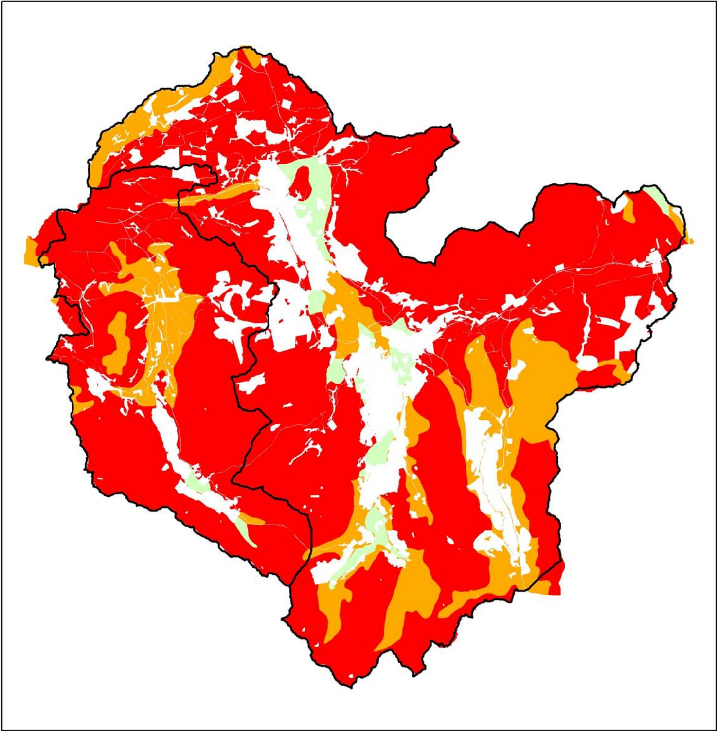
Map 19 Priority soils for woodland creation in the wider catchment to reduce surface runoff and/or sediment delivery to watercourses
